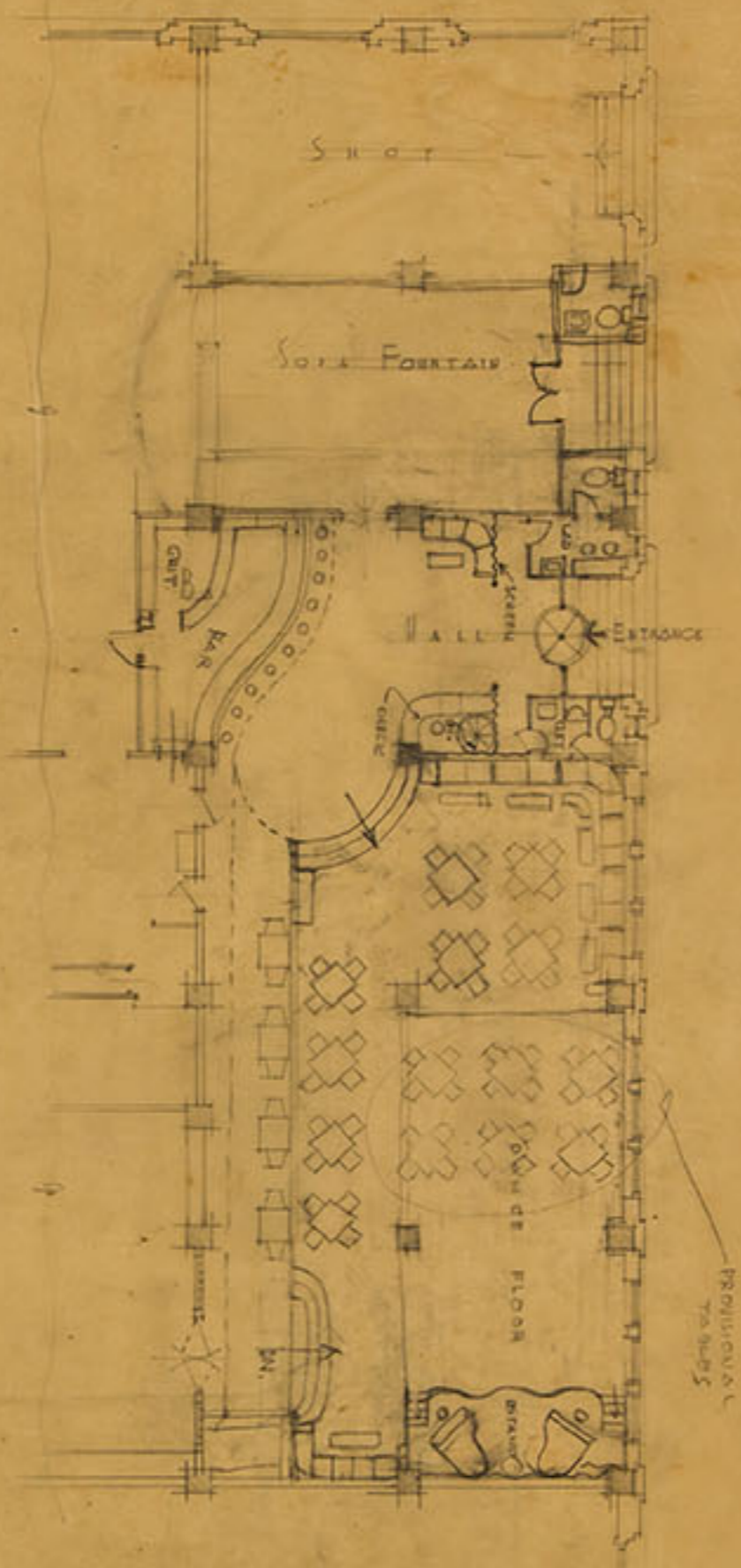
• CANTERIA FLOOR PLAN • GROUND FL., PENINSULA HOTEL SCALE: 1/8" = 1'-0"
