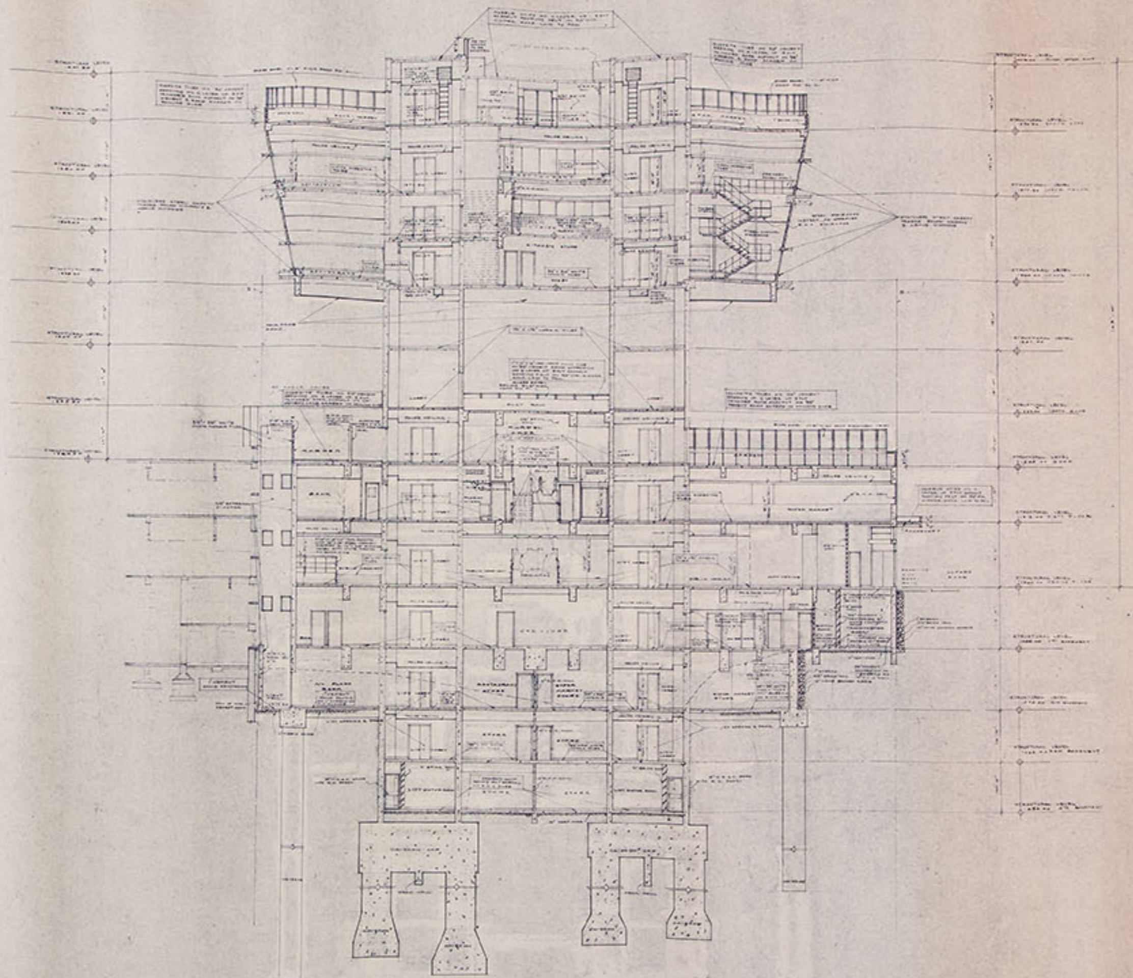
SECTION C-C
